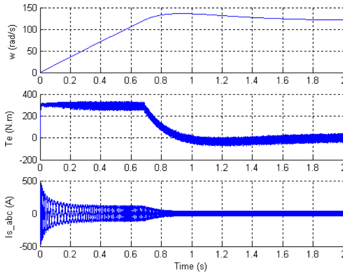
Starting the Induction Motor Drive
